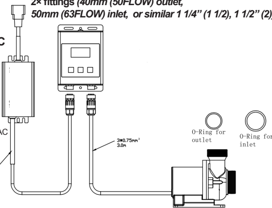
Schematic of connection of the Red Dragon® 5 ECO
