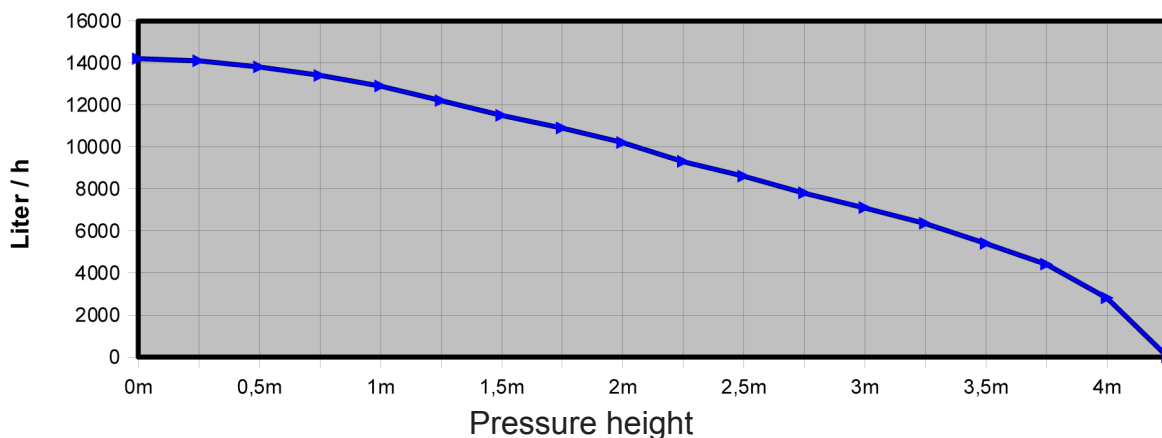
Power curve
