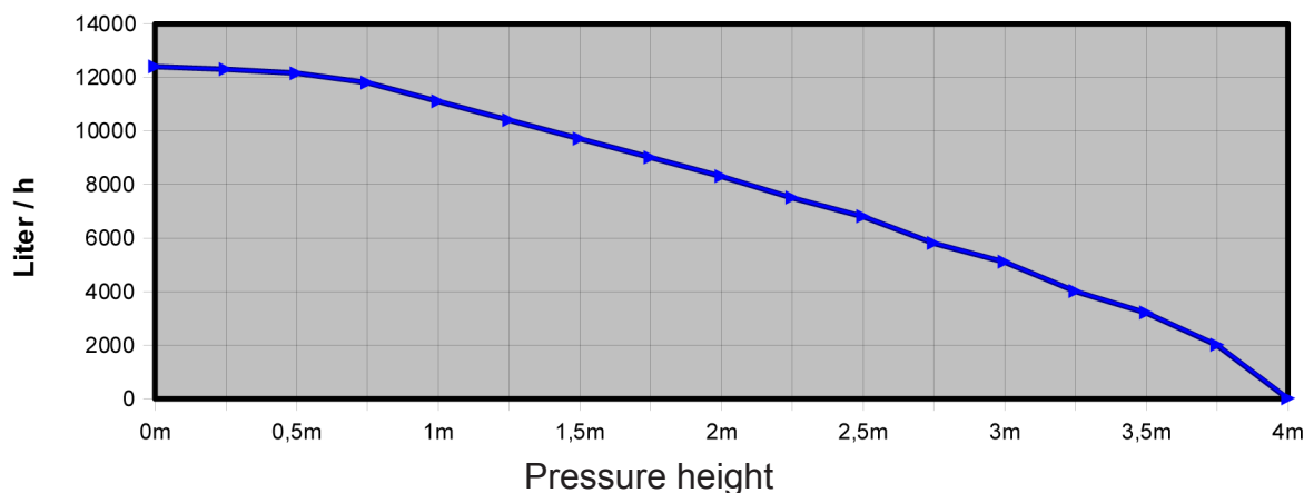
Power curve
