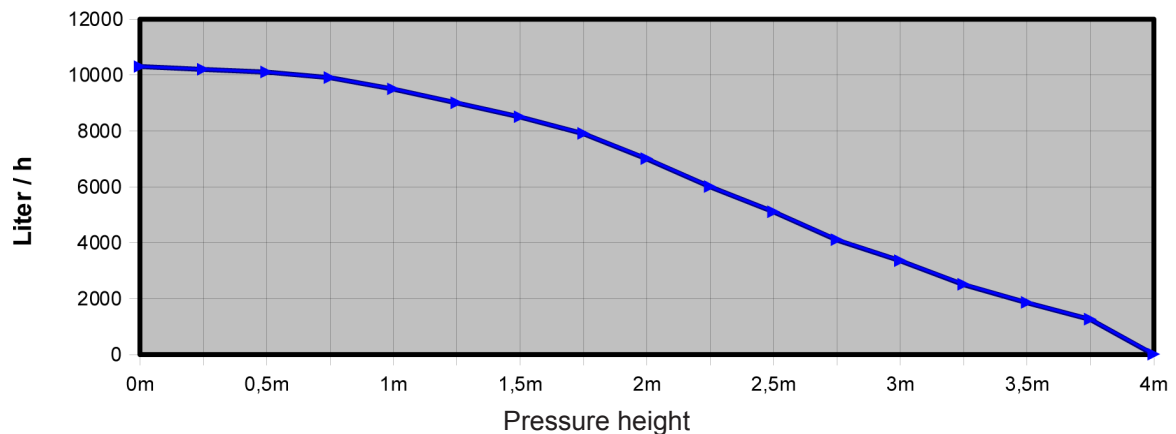
Power curve
